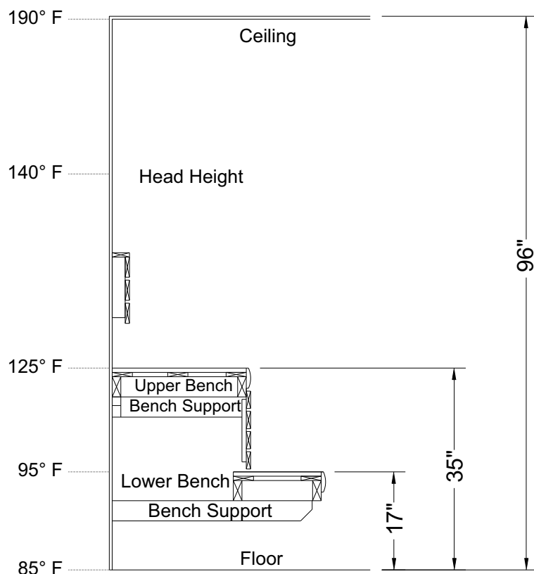
DIAGRAM 14: ROOM TEMPERATURES
