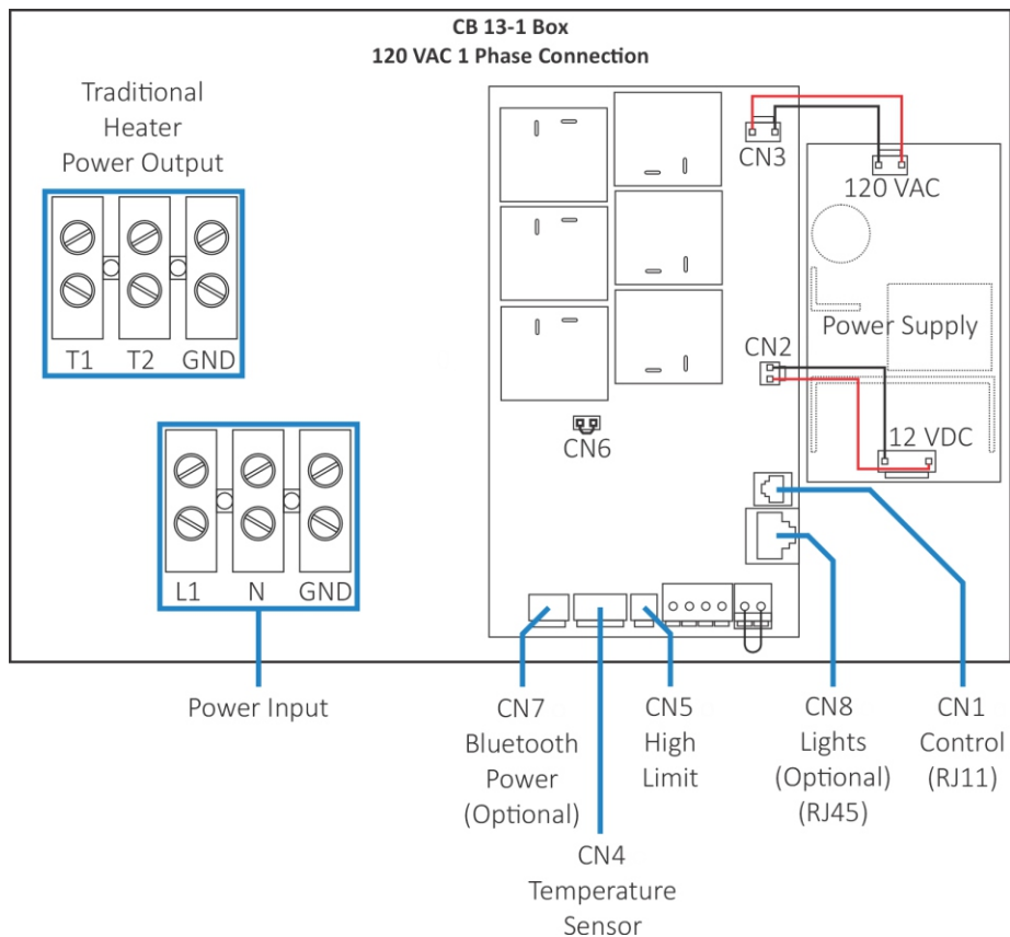
DIAGRAM 7: CB BOX INTERNAL VIEW
