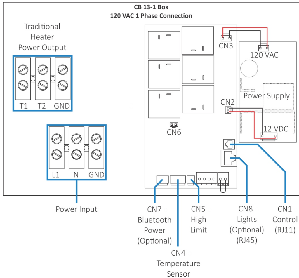
DIAGRAM 6: CB BOX INTERNAL VIEW
