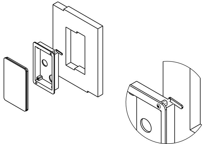
DIAGRAM 8: SL2 MOUNTING
