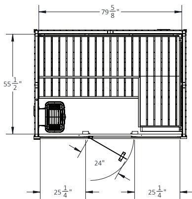
Top Down View w/ Interior Measurements
